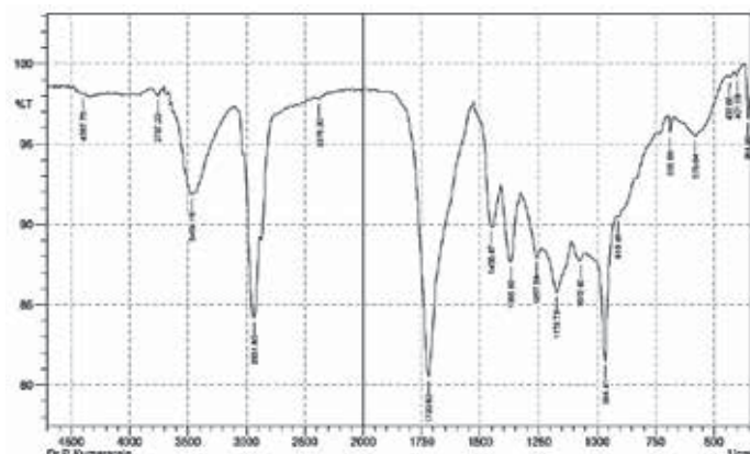
FT-IR Characterisation of E2 active component
