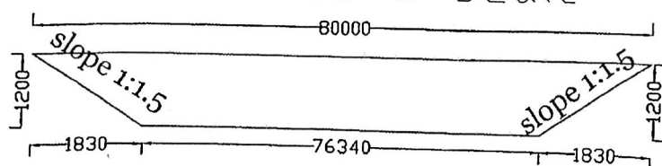
Cross section Not to a Scale
